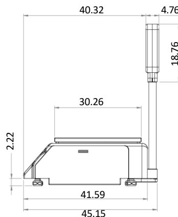
Vista frontal
